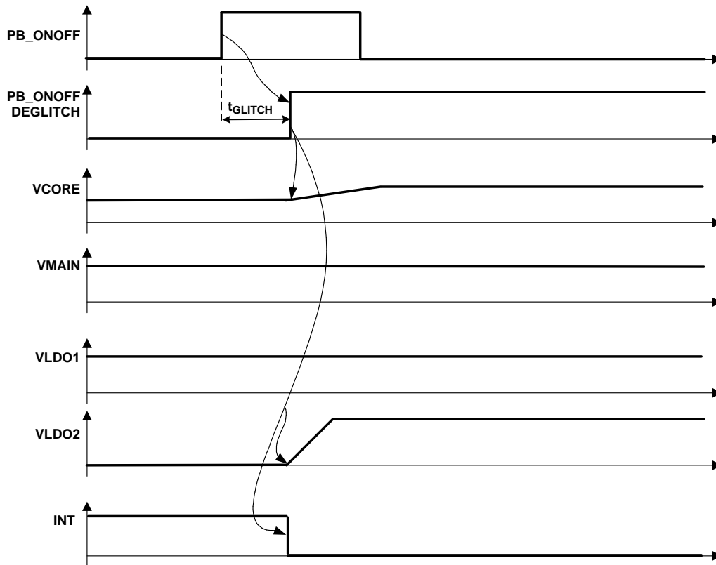
Figure 34. State 3 to State 2 Transition. PB_ONOFF Activated (See Interrupt Management Section for \overline{INT} Behavior)
